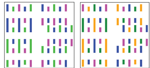
SADP/SAQP fill and cut
